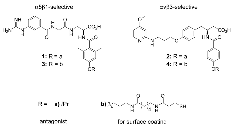
Scheme 1. \alpha 5 \beta 1 -Selective ( 1 ) and \alpha \nu \beta 3 -selective ( 2 ) integrin antagonists and their thiol-functionalized analogues ( 3 , 4 ) for binding to gold nanoparticles.
