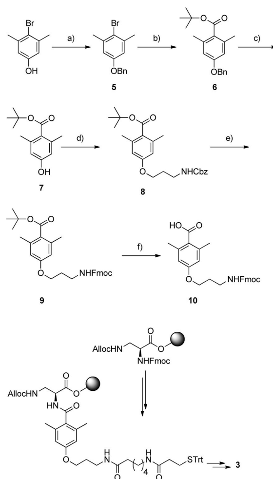
Scheme 2. Synthesis of building block 10 and functionalization of the \alpha 5 \beta 1 -selective integrin antagonist on a solid support, yielding thiol 3 . a) NaH, 0 °C, DMF; BnBr, RT; b) n BuLi, −78 °C, THF; Boc 2 O, RT; c) H 2 , [Pd/C], MeOH; d) 1,1'-(azodicarbonyl)dipiperidine, PBu 3 , THF; e) H 2 , [Pd/C], MeOH; Fmoc-OSu, NaHCO 3 , THF/H 2 O; f) TFA/triisopropylsilane/H 2 O 95/2.5/2.5. Alloc = allyloxycarbonyl, Bn = benzyl, Boc = tert -butoxycarbonyl, Cbz = carboxybenzyl, TFA = trifluoroacetic acid, Trt = trityl.
